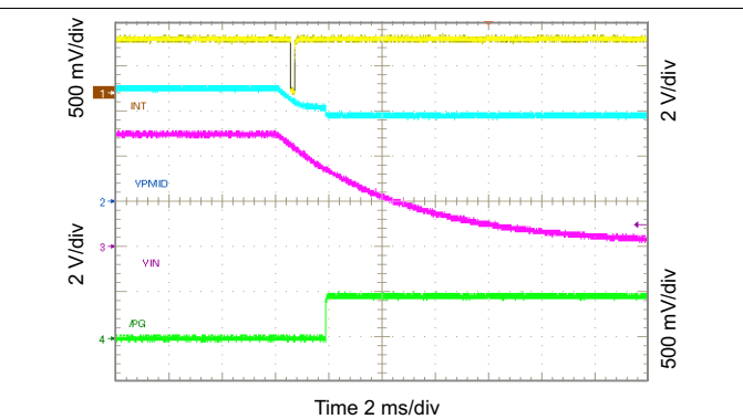
Figure 94. Show \overline{\text{PG}} and \overline{\text{INT}} Timing ( \text{VIN} Removal)
